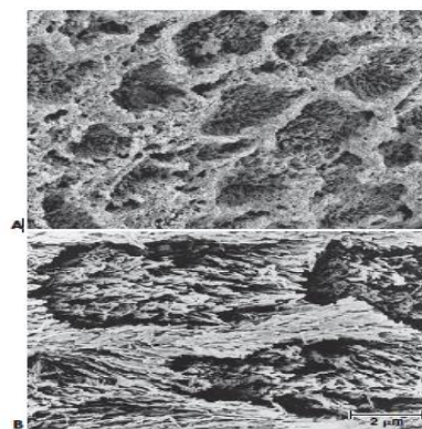
Figure 6: SE micrograph of enamel etched with 35% phosphoric acid for 15 seconds, denoting a type I etching pattern in A. Type III etching pattern in B.
