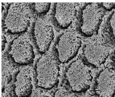
Figure 4: Scanning electron micrograph of enamel etched with 35% phosphoric acid for 15 seconds.
