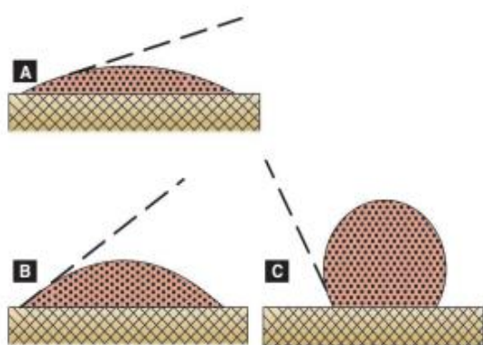
Figure 1: Degree of contact angle influences the wetting of surface; (A) when contact angle is small, wettability of the adhesive is better; (B) and (C) When contact angle is large, liquid does not wet the surface completely.
