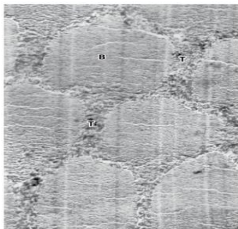
Figure 3: Electron micrograph of mature human enamel shows keyhole-shaped rods with differing crystal orientation in the body (B) and tail (T).
